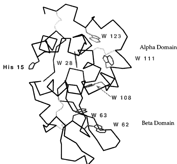
FIGURE 1: Hen egg white lysozyme. A C \alpha backbone trace and the histidine, tryptophan, and cystine residues are shown (PDB file 8LYZ; Beddell et al. , 1975).
