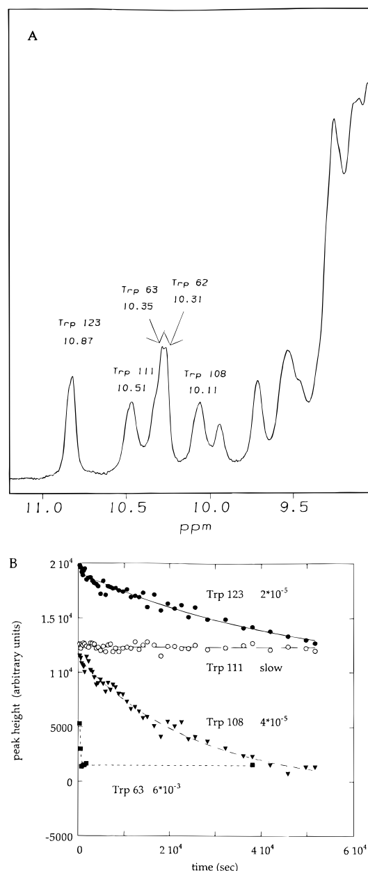
FIGURE 4: Native state hydrogen exchange of lysozyme tryptophan indole nitrogen protons. (A) 1D ^1\text{H} -NMR spectrum of lysozyme recorded in H_2O at pH 4.0 with 100 mM NaCl, 50 mM NaAc, and no GdmCl at 10 °C showing the presence of the Trp indole nitrogen proton peaks. (B) The exchange rates of the Trp indole nitrogen protons from folded lysozyme in D_2O at pH* 4.0 with 100 mM NaCl, 50 mM NaAc, and no GdmCl at 10 °C. The identity and exchange rate in units of \text{s}^{-1} are given.
