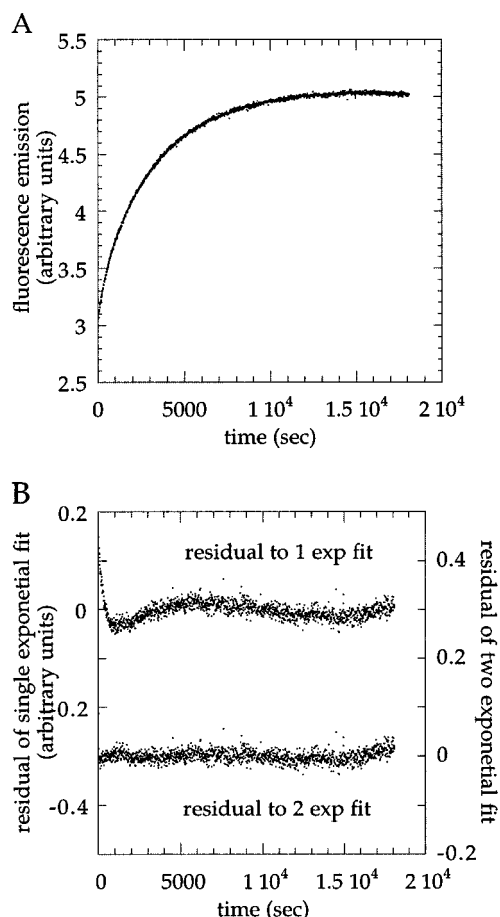
FIGURE 3: Unfolding kinetics of lysozyme followed by ultraviolet fluorescence emission. (A) Lysozyme unfolding at pH* 4.0 in 6.00 M GdmCl, 100 mM NaCl, and 50 mM NaAc in D_2O at 10.0 °C. The excitation wavelength was 295 nm, and the emission wavelength was 350 nm. The experimental data are fitted by a two-exponential equation. (B) The residual plots to one- and two-exponential fits of this data.
